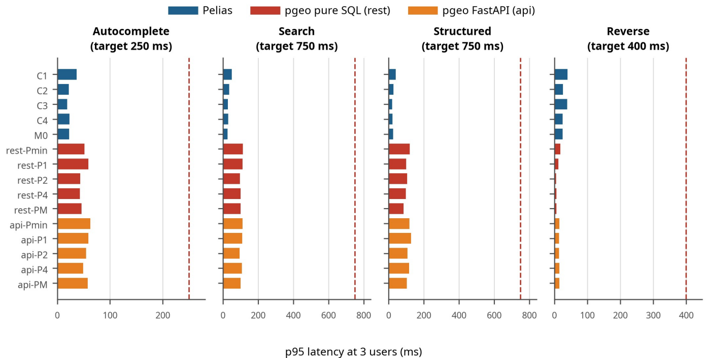
Figure 12. p95 latency per endpoint at 3 users for each configuration, against its target (dashed). Every configuration of both engines meets every target.
