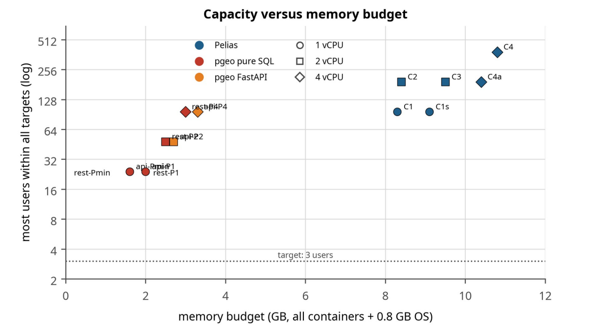
Figure 1. Capacity against memory budget for every tested configuration of both engines. Each point is one configuration; the vertical axis is the most concurrent users for which every endpoint stayed within its latency target (log scale). pgeo configurations sit at the left (1.6-3.3 GB), Pelias at the right (8.3-10.8 GB). The dotted line is the project’s 3-user goal.
