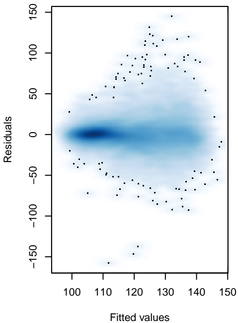
Linear Age + Gender + BMI
