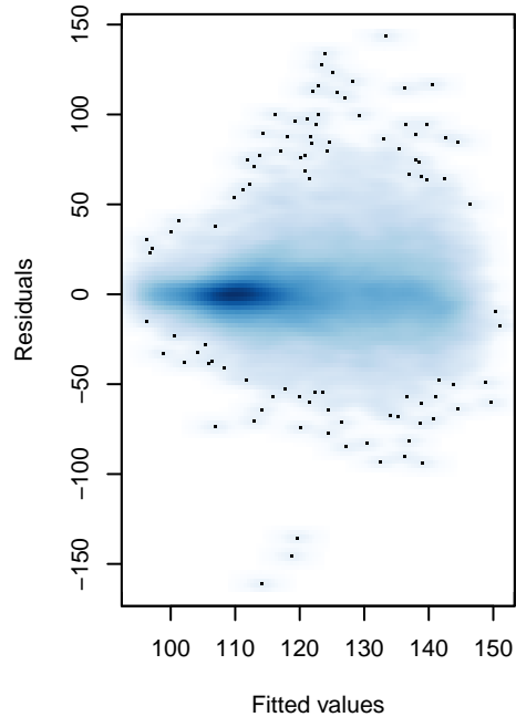
Spline Age + Gender + BMI
