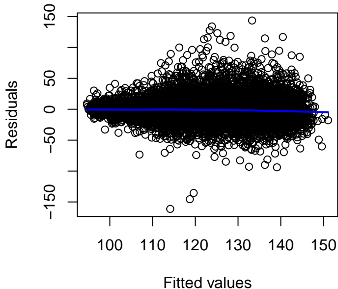
Spline Age (no interaction on SBP)
