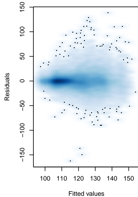
Spline Age \times Gender + BMI
