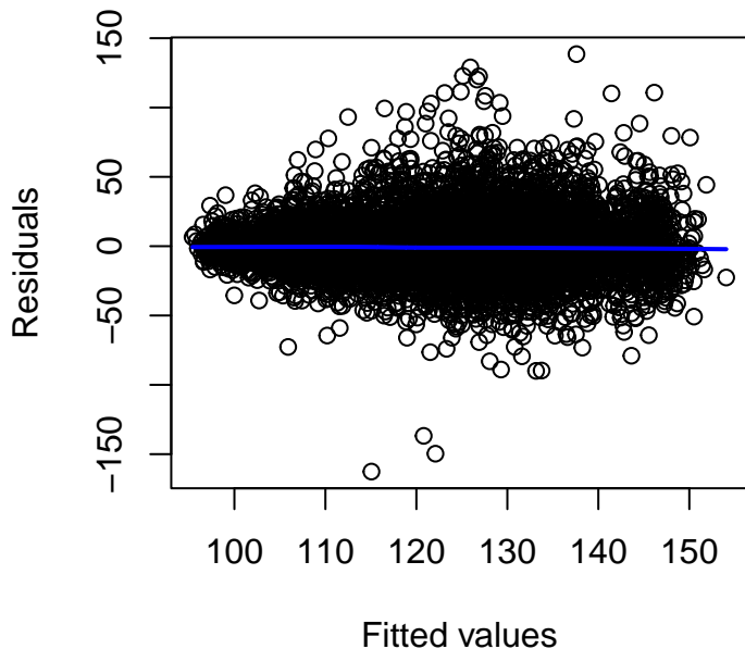
Spline \times gender Interaction on SBP
