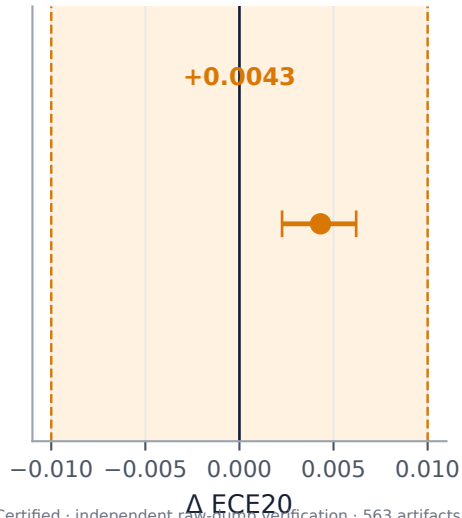
c Calibration shifts modestly
