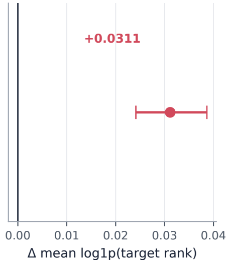
a Ranking worsens
