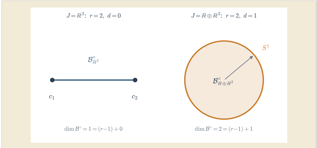
FIG. 3. Two rank-2 carriers, so two weights in each case. On the left the extreme points are two isolated vertices and the interval is entirely weight; on the right they sweep a circle, and the frame contributes one dimension the weights cannot see.
