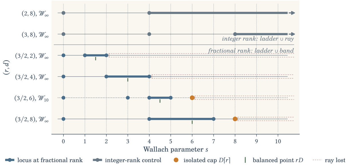
Figure 4. Positivity at integer and fractional rank; each row is labelled with the locus it shows, and the one finite-cutoff row carries a dashed rule. The grey integer controls ( r = 2, 3 ), governed by Theorem 8.5, carry the classical ladder and an unbounded ray. Every fractional row has r = 3/2 , and its ray is replaced by a bounded band whose erosion is decided by the defect v = d/4 : none at d = 2, 4 , one step at d = 8 before the rank-null ideal halts it, two-sided at d = 6 , where no ideal exists. An amber mark is an isolated cap point D[r] , retained at every degree by Proposition 9.3 and maximal in its locus by (82); the short rule beneath each fractional row is the balanced point rD of (72), which every band contains. All loci are exact. Every fractional row has d even, so Theorem 9.9(i)–(iii) applies; see Remark 9.1 for odd d .
