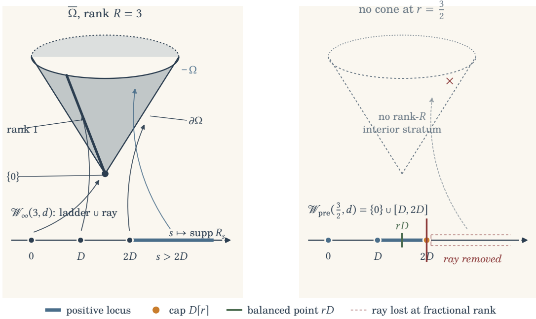
Figure 3. The geometric dictionary, and what survives without it. Left: at integer rank R = 3 the Riesz distribution R_s is a positive measure exactly on the Wallach set, and at the ladder point s = jD its support is the closure of the rank- j orbit [6, Prop. VII.2.3, Thm. VII.3.1]. The map s \mapsto \text{supp } R_s therefore carries the ladder onto the flag \{0\} \subset \overline{\mathcal{O}}_1 \subset \partial\Omega and carries the unbounded ray onto the interior \Omega ; the arrows are that map, and the cone is a perspective drawing in which only the containment order is meaningful. Right: at r = \frac{3}{2} there is no cone, hence no interior stratum for a ray to be supported on. What Theorem 9.1 and Proposition 9.3 leave is the left-hand end of the picture — the retained grid \{0, D, 2D\} and the bounded band \mathcal{W}_{\text{pre}} = \{0\} \cup [D, 2D] containing the balanced point rD , capped at D[r] by (82). The channel to the right of the cap is where the ray was. The band shown is the pre-erosion locus of Theorem 9.1; at d = 6 and d = 8 it subsequently erodes, as Table 1 records.
