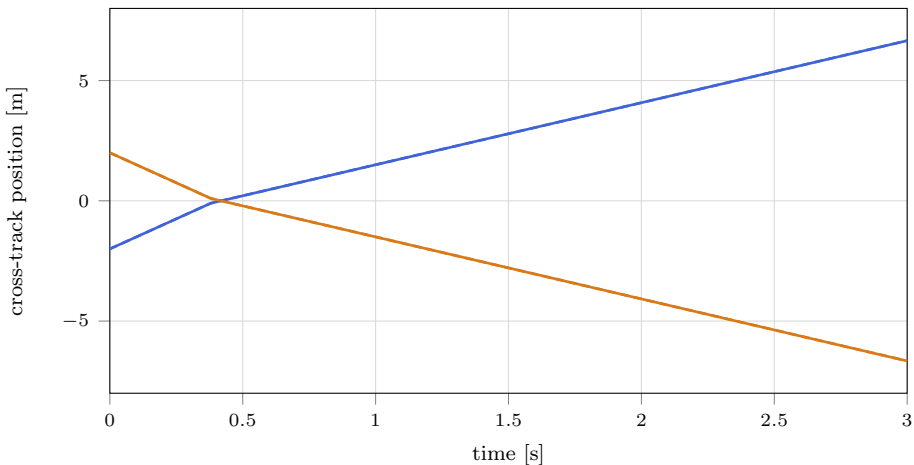
Full chief orbit: naive zero-g drifts; mujoco_orbit returns
