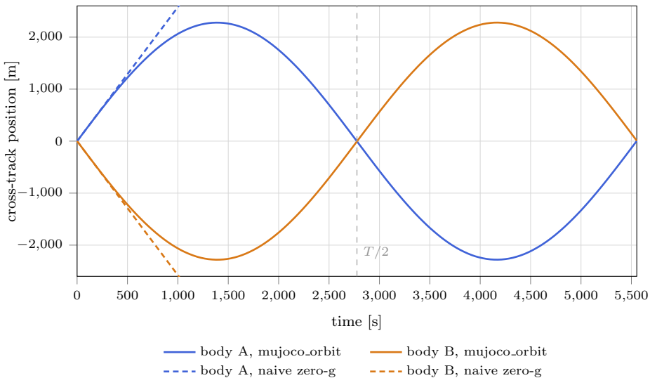
Full chief orbit: naive zero-g drifts; mujoco_orbit returns
