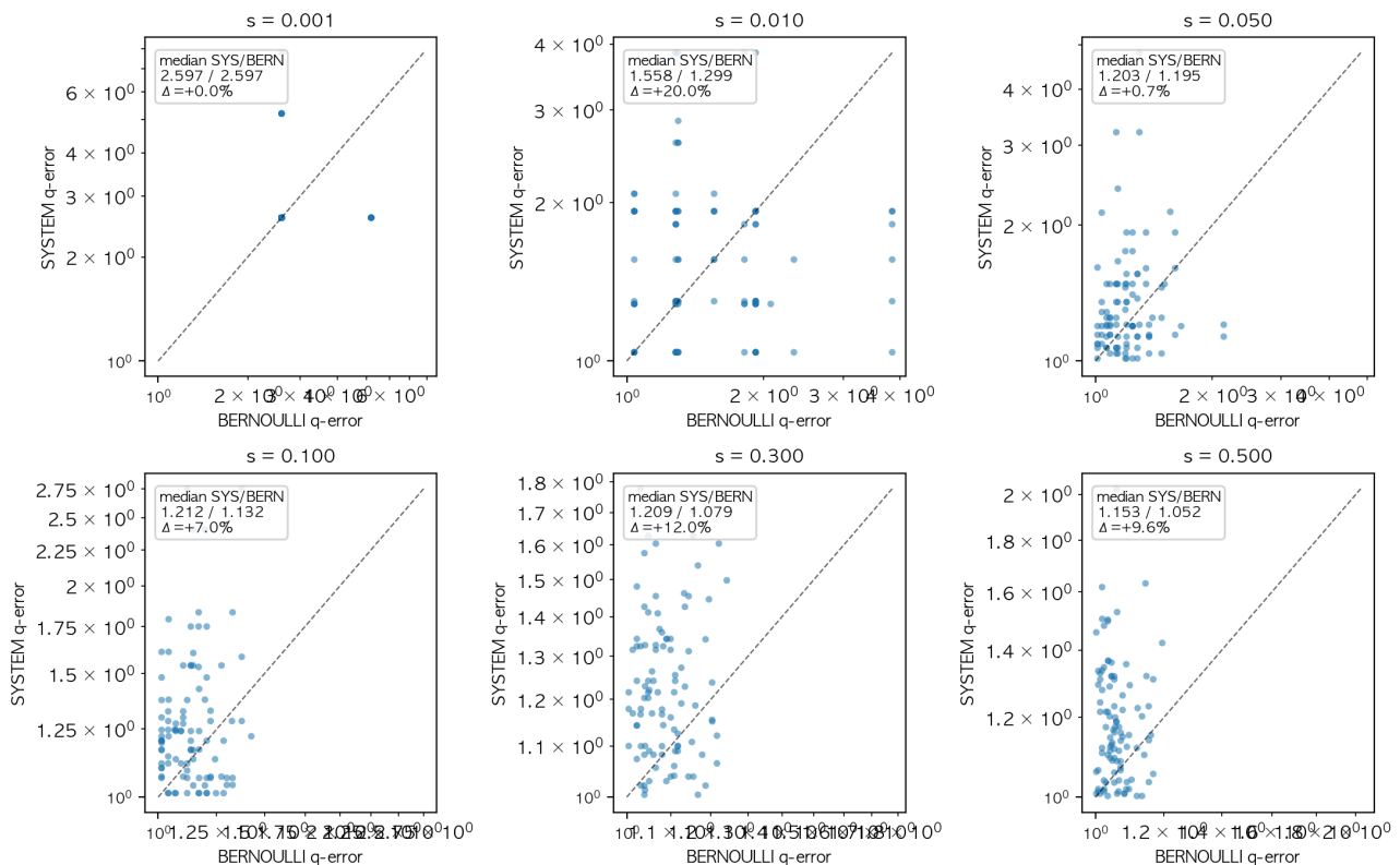
Figure 1 — Phase 4 Native SYSTEM vs BERNOULLI (100 query paired, 6 selectivity)
