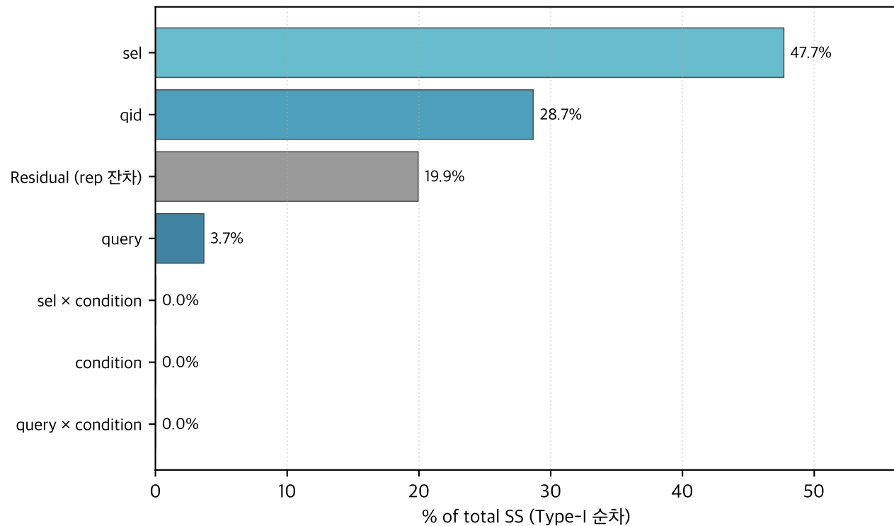
(b) baseline 제외 — n=2,115 , R^2=0.801
