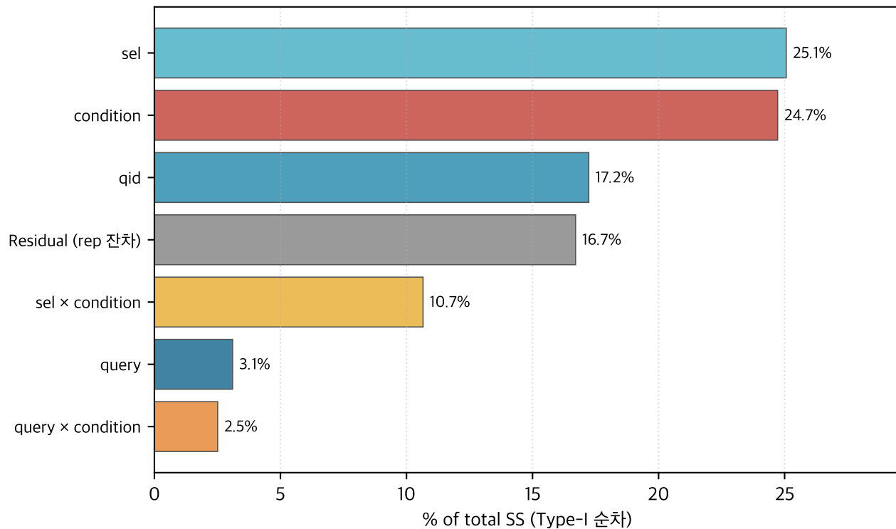
(a) 4 condition (baseline·B1·CaseB·oracle) — n=2,910 , R^2=0.833
