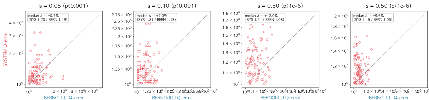
Phase 4 — SYS vs BERN paired Q-error 4 panel ( s=0.05/0.10/0.30/0.50 )
