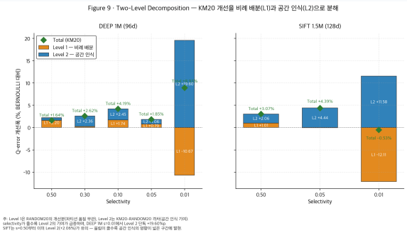
Two-Level Decomposition — Level 1 (비례) + Level 2 (공간 인식) 분해
