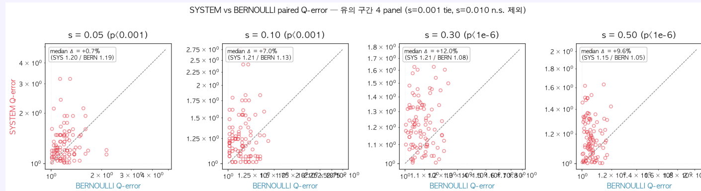
Phase 4 — SYS vs BERN paired Q-error 4 panel ( s=0.05/0.10/0.30/0.50 )
