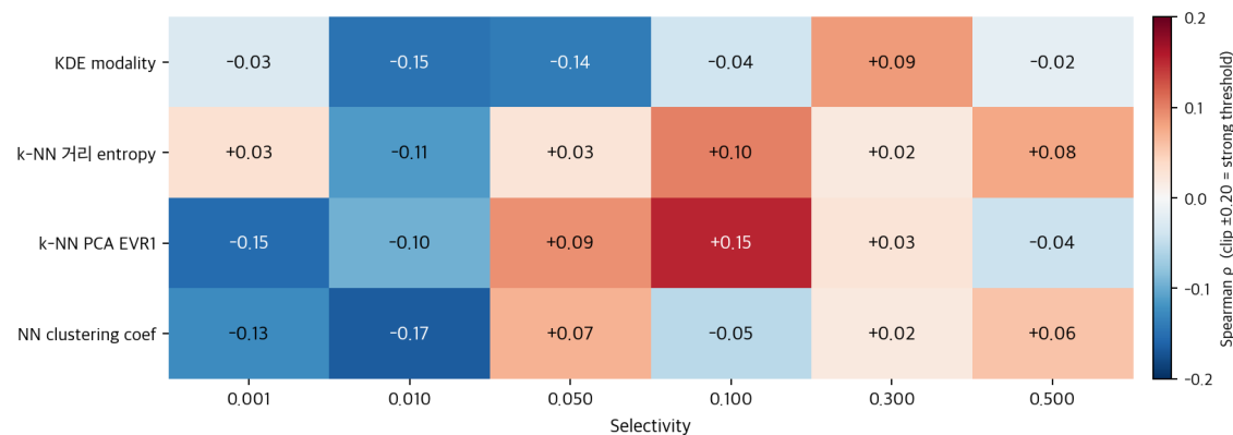
Figure 6 · Phase 5 Local Skew × Q-error Spearman \rho — 모든 조합 |p| < 0.2 (negative result)
