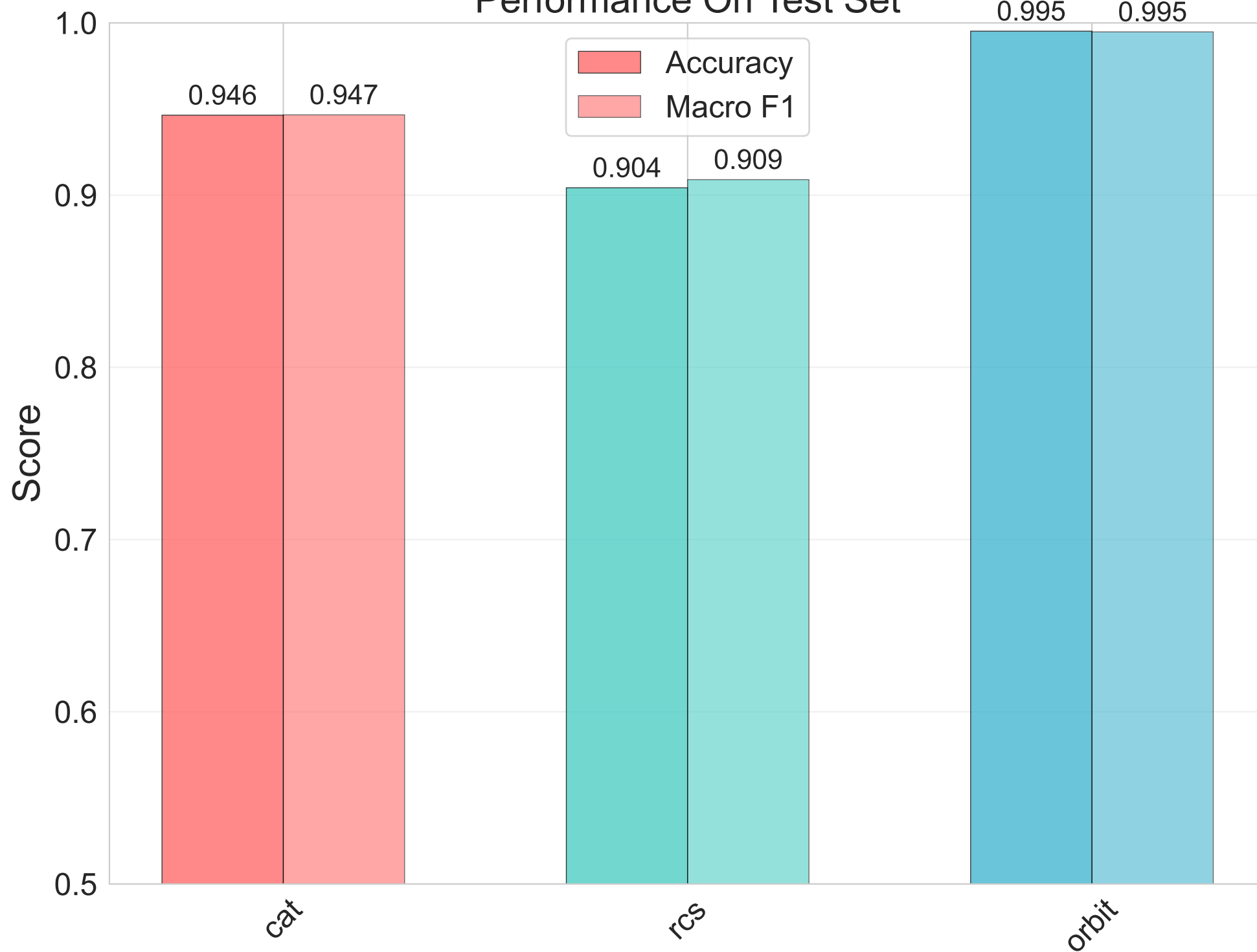
Performance On Test Set
