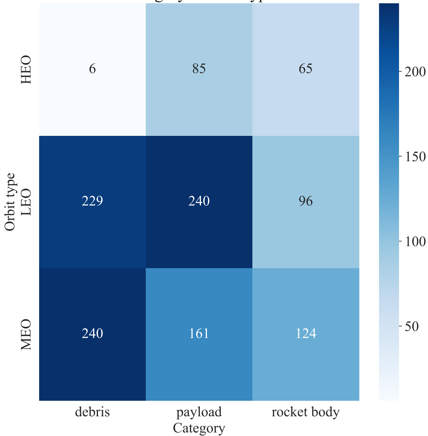
Category \times Orbit type
