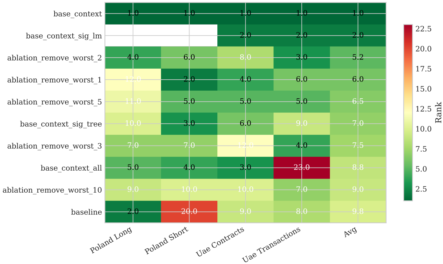
Strategy Ranking Heatmap (Lower is Better)
