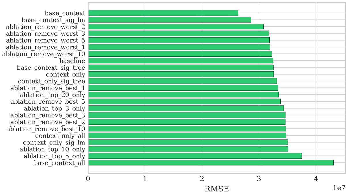
Sales Uae Transactions: Strategy RMSE Ladder
