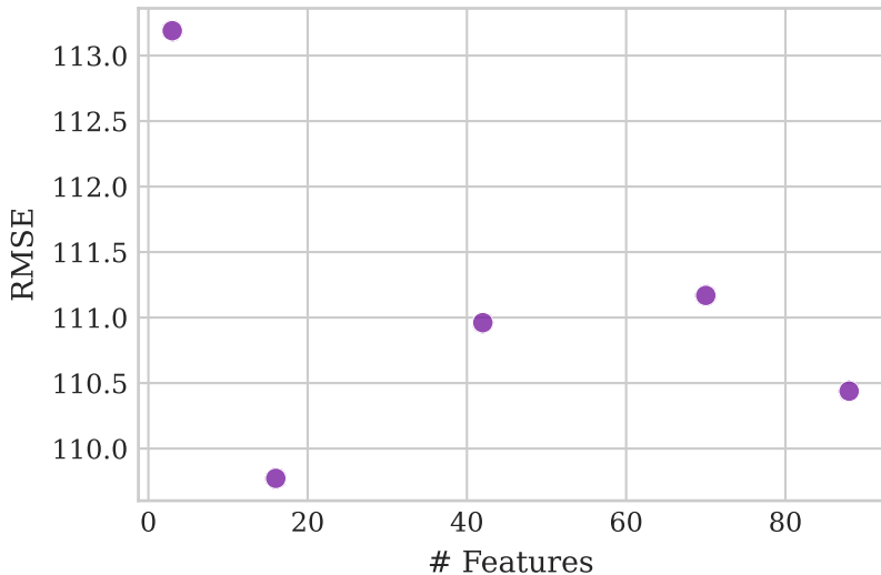
M5 Store Dept Daily: Feature Ablation
