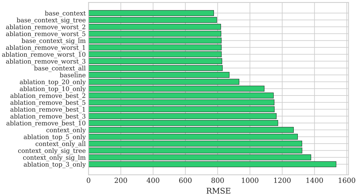
Rossmann Daily: Strategy RMSE Ladder
