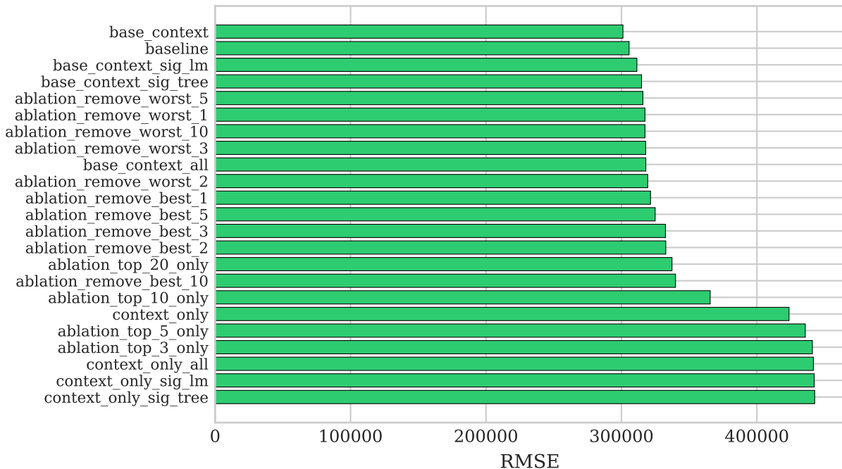
Melbourne Housing: Strategy RMSE Ladder
