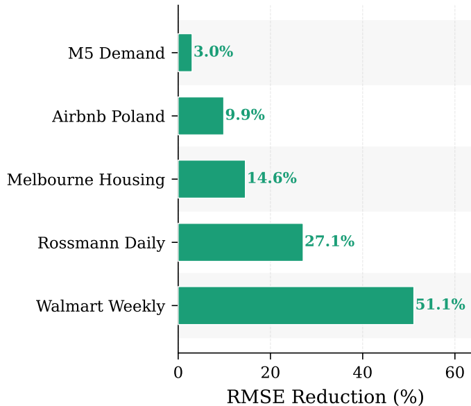
(a) Best RMSE Improvement
