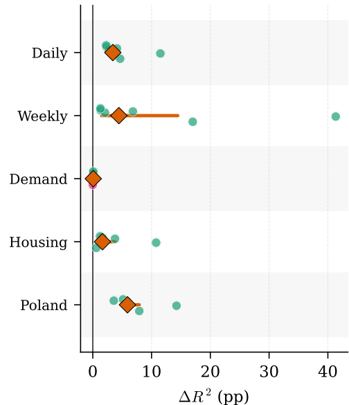
(c) R^2 Improvement
