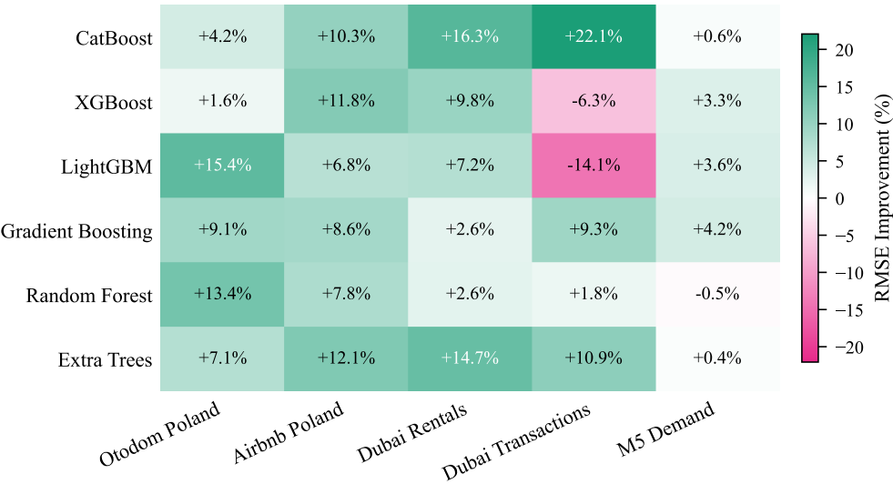
RMSE Improvement (%) by Model and Dataset
