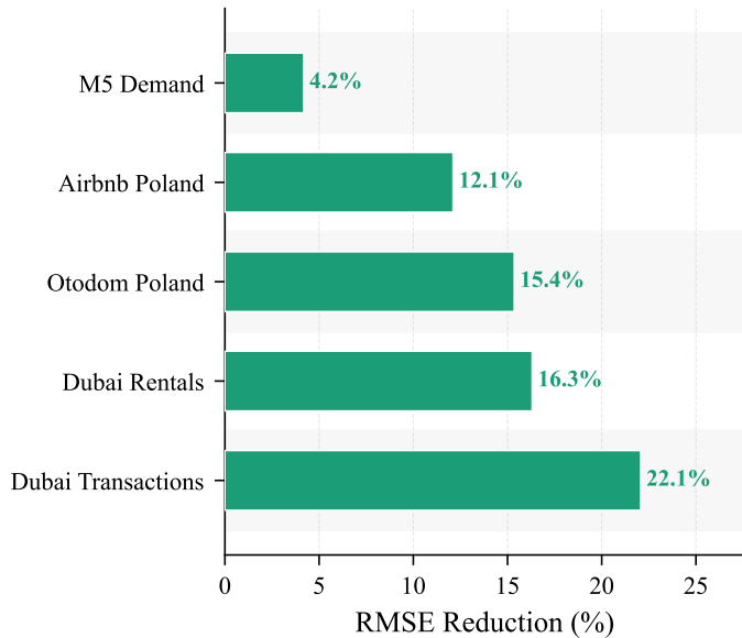
(a) Best RMSE Improvement
