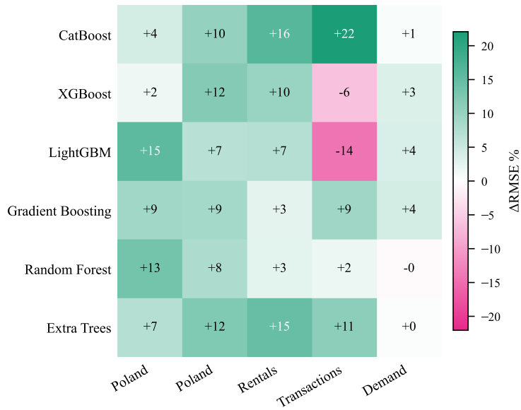
(b) RMSE Improvement by Model
