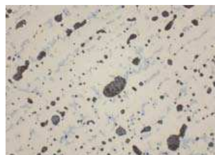
Fig. 17: Bronze cast, CuSn8Pb, unetched, large and small blue-grey lead inclusions, pale blue \alpha - \delta eutectoid discernable, 500x.
