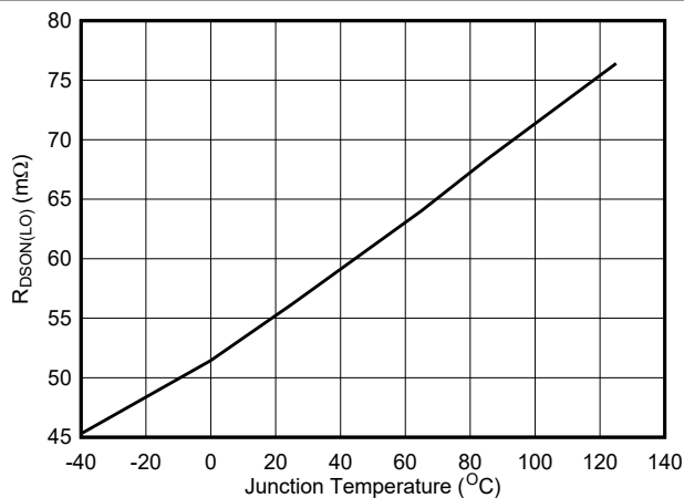
Figure 5-5. Low-Side R_{\text{dson}}
