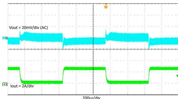
Figure 7-20. TPS563203 Load Transient With 0.3A to 2.7A
