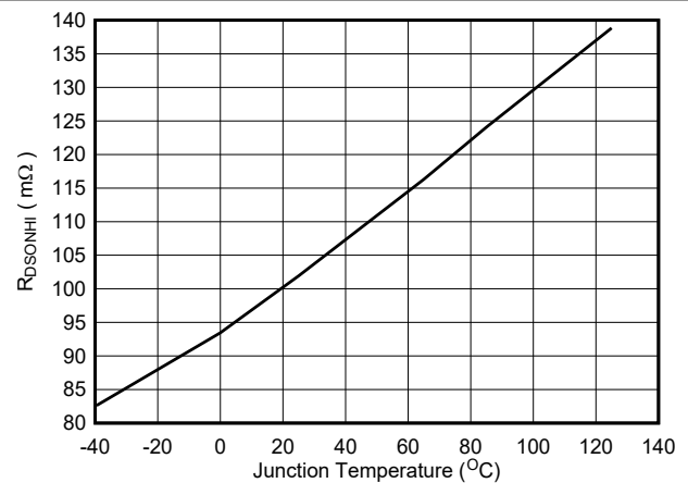
Figure 5-6. High-Side R_{\text{dson}}
