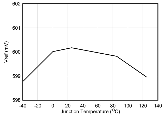
Figure 5-2. V_{\text{ref}} Voltage
