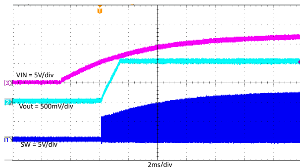
Figure 7-16. TPS563203 Power on With 3A Loading
