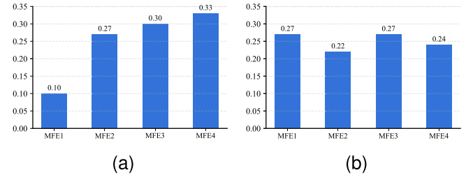
Fig. 11. Statistical analysis of the probability of selecting each expert without and with L_{aux} . (a) Without L_{aux} . (b) With L_{aux} .
