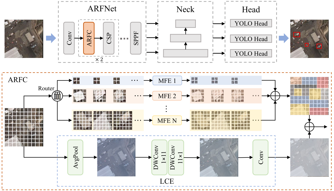
Fig. 2. Architecture of the proposed ARFN-MoE, where our ARFC module replaces a conventional convolution in the backbone. The ARFC is comprised of a grid-level router and a set of MFE.
