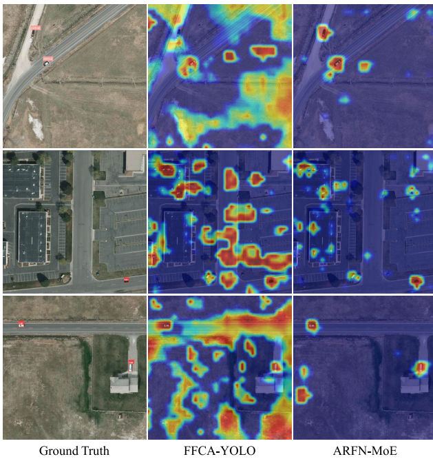
Fig. 8. Grad-CAM visualization of heatmaps generated by our proposed ARFN-MoE and the state-of-the-art FFCA-YOLO on the VEDAI dataset.
