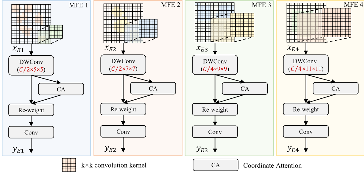
Fig. 4. Structure of the MFE. It comprises four experts with varying kernel sizes and channel numbers to extract optimal features for multiscale small objects.
