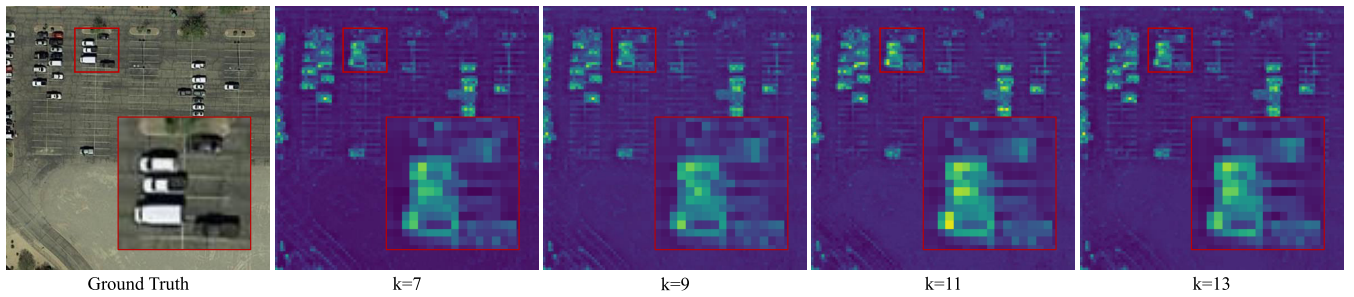
Fig. 10. Visualize the output features of LCE with different kernel sizes. It can be observed that the highest attention to small objects occurs when the kernel size is 11, at which point LCE can more effectively extract the features of small objects.
