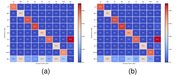
Fig. 5. Comparison of the confusion matrix between our ARFN-MoE and FFCA-YOLO on the AI-TOD dataset. (a) FFCA-YOLO. (b) Ours.
