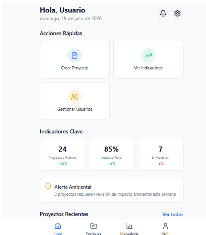
Figura 2. Mockup - Panel principal
