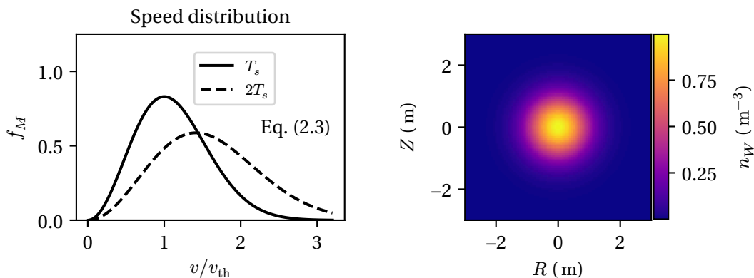
Figure 2.1 – Left: the speed distribution f_M of Eq. (2.3), at two temperatures. Right: some heatmap figure that doesn't slow down pdf readers.
