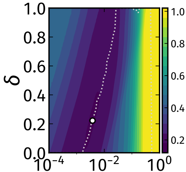
rhee2006
