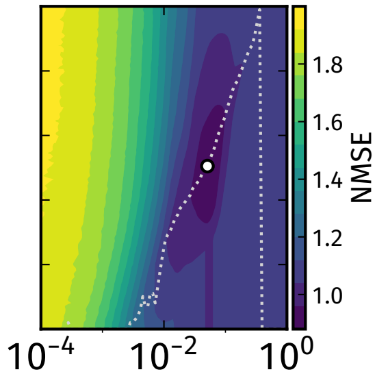
triazines
