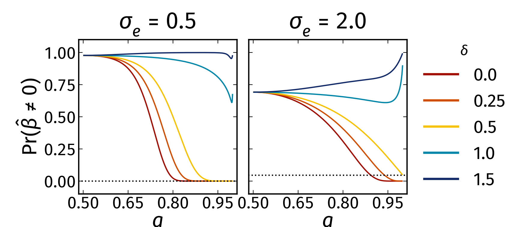
Figure 2: Lasso selection probability vs. class balance q for several \delta . Dotted line: asymptotic limit at \delta = \frac{1}{2} .
