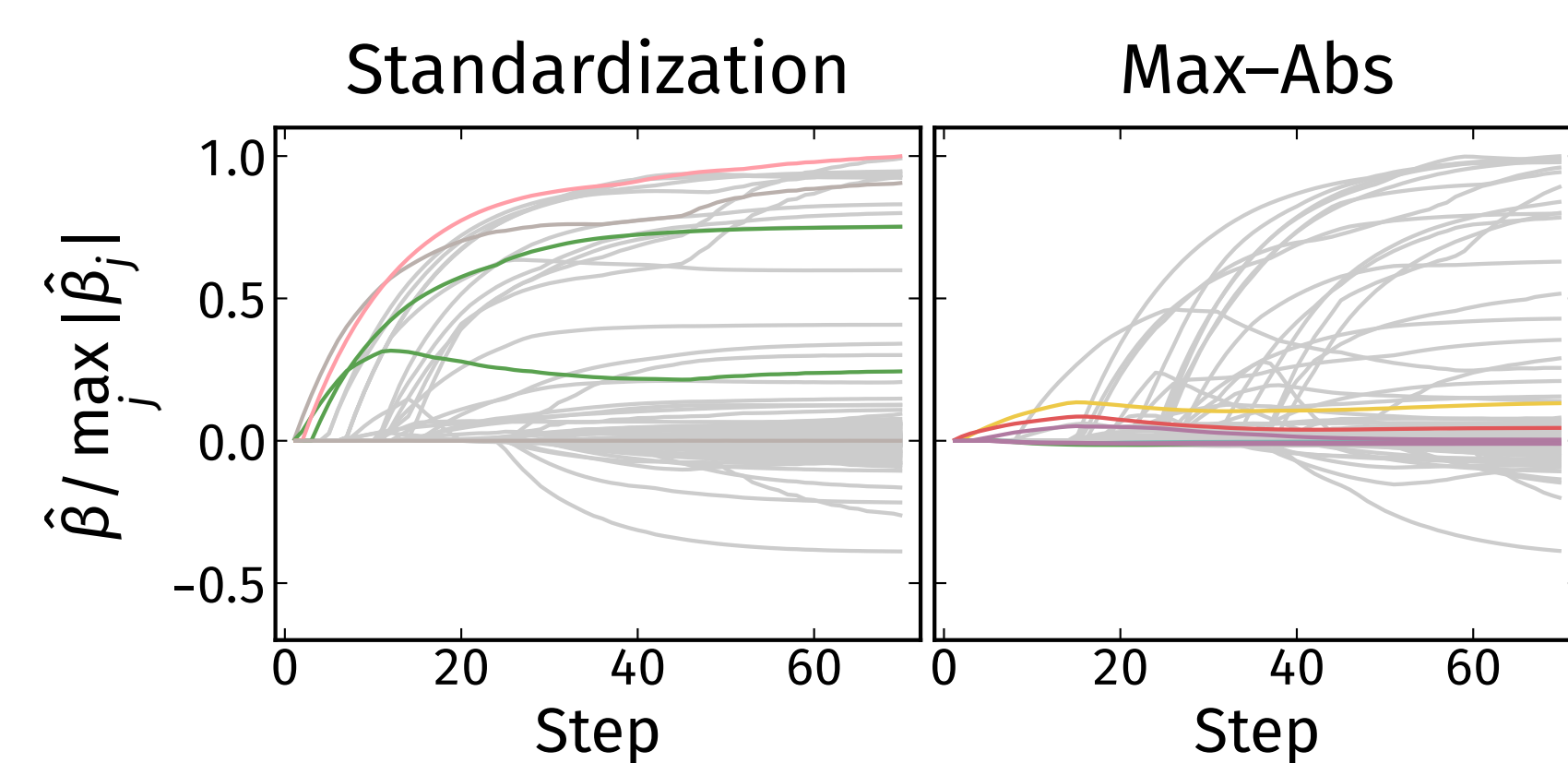
Figure 1: Lasso paths for w1a under standardization ( \delta = 0.5 ) and max-abs ( \delta = 0 ), with first features to enter highlighted.
