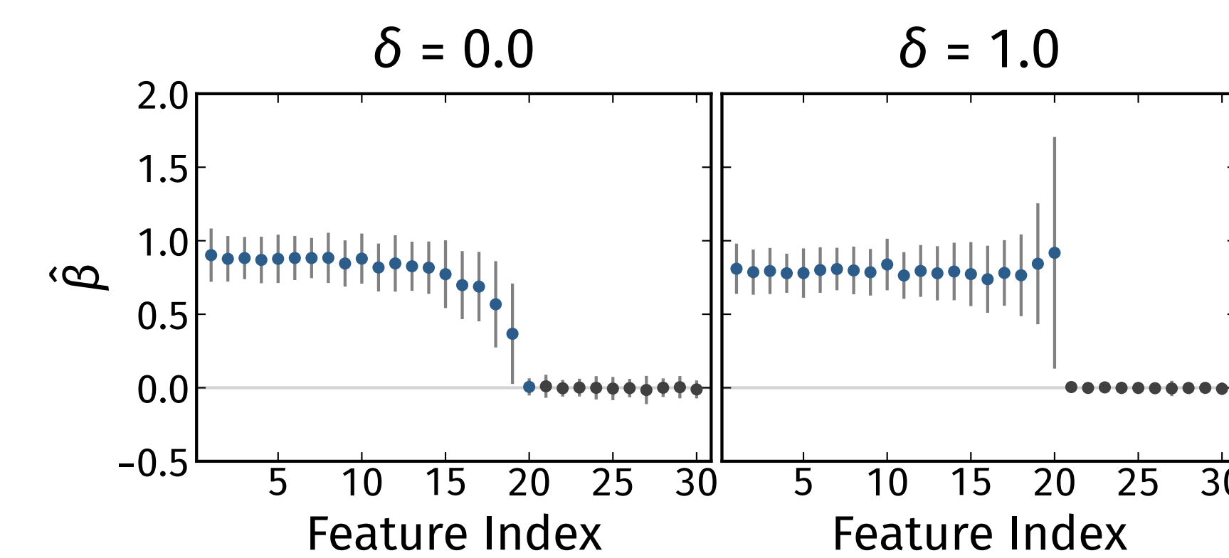
Figure 3: Lasso estimates (mean \pm SD) for a simulation with p = 1000 (the first 20 features are signals with class balance 0.5 \rightarrow 0.99 ; first 30 shown). No scaling drops the imbalanced signals; variance scaling recovers them.
