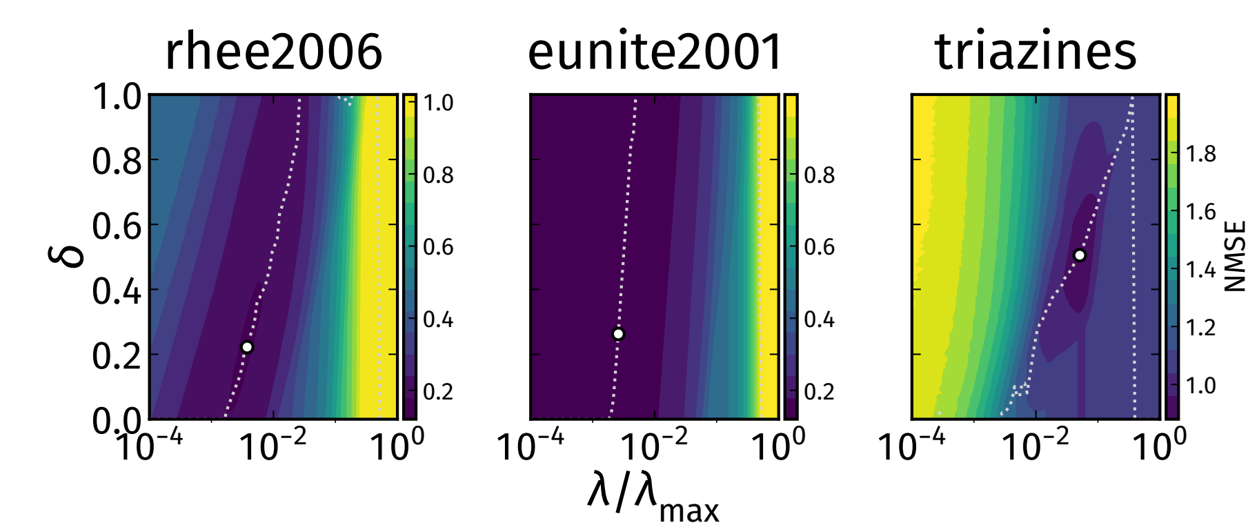
Figure 4: Hold-out (validation) NMSE over (\lambda, \delta) for the lasso on three data sets. White dot: tuned optimum; dotted line: best \delta at each \lambda . The optimal \delta is interior and data set-dependent.
