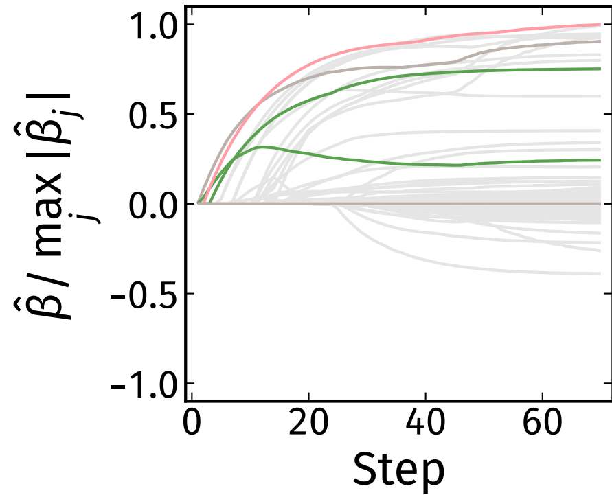
Standardization
