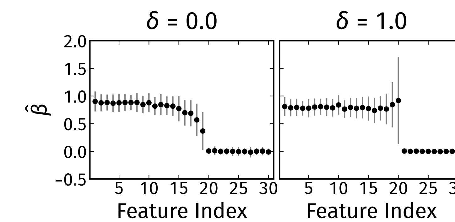
Figure 3: Lasso estimates (mean \pm SD) for a simulation with p = 1000 (the first 20 features are signals with class balance 0.5 \rightarrow 0.99 ; first 30 shown). No scaling drops the imbalanced signals; variance scaling recovers them.
