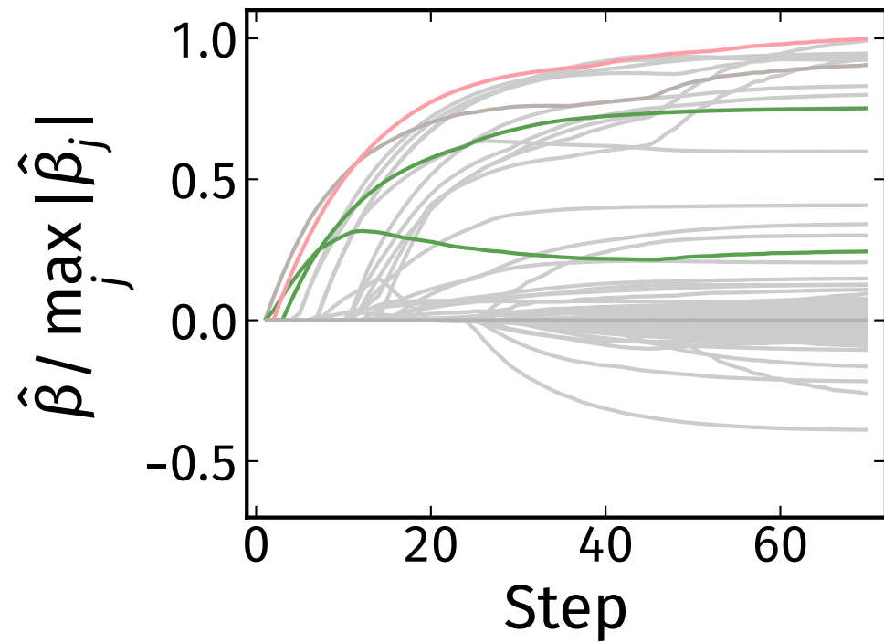
Standardization
