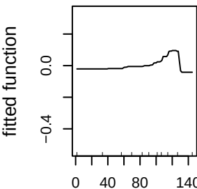
aspect_sd_50m (4.8%)
