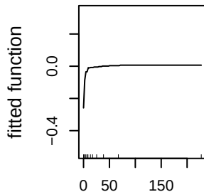
max_curv_30m_sd_50m (6.6%)
