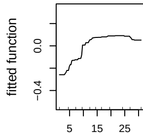
depth_mean_50m (10.2%)
