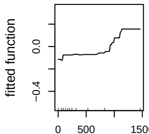
max_sos_30m_sd_50m (4.4%)
