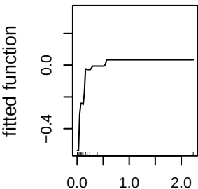
rugosity_sd_50m (18.1%)
