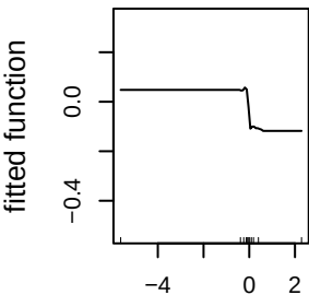
curvature_mean_50m (6.7%)
