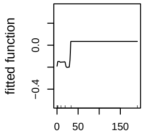
max_curv_30m_sd_50m (6.6%)
