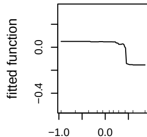
aspect_cos_50m (6%)
