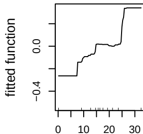
sos_sd_50m (14.6%)
