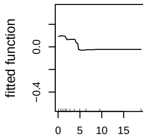
max_sos_30m_sd_50m (4.4%)
