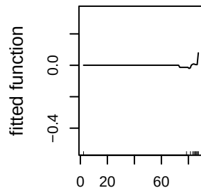
ax_sos_240m_mean_50m (4.3%)
