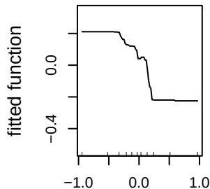
aspect_sin_50m (14.5%)
