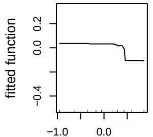
aspect_cos_50m (6.1%)
