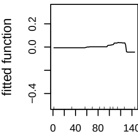
aspect_sd_50m (3.9%)
