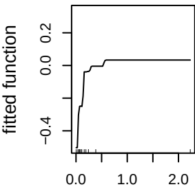
rugosity_sd_50m (23.1%)
