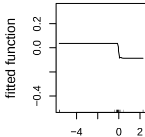
max_curv_30m_sd_50m (8.8%)
