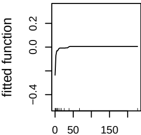
max_curv_30m_sd_50m (8.8%)
