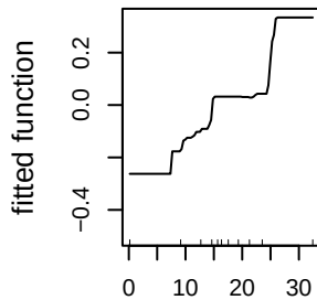
sos_sd_50m (21.2%)
