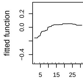
depth_mean_50m (8.8%)
