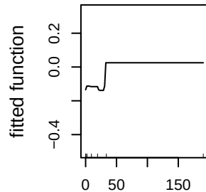
max_curv_240m_sd_50m (3.9%)
