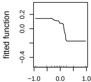
aspect_sin_50m (15.2%)
