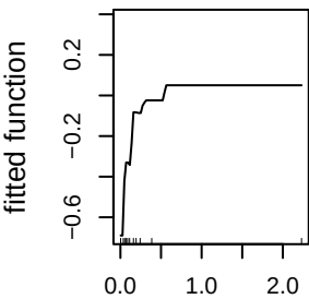
rugosity_sd_50m (27.9%)
