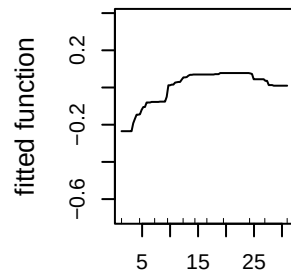
depth_mean_50m (11.9%)
