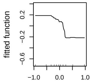
aspect_sin_50m (17.3%)
