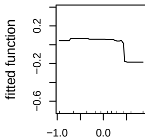
aspect_cos_50m (9.5%)
