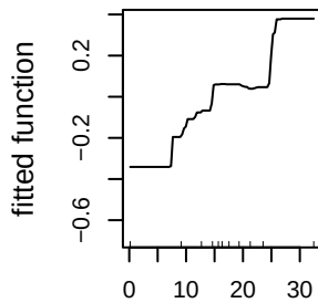
sos_sd_50m (23.4%)
