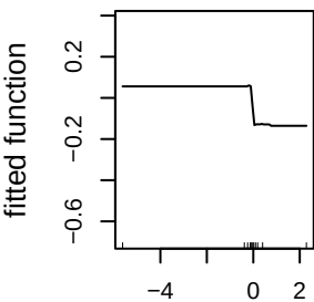
curvature_mean_50m (10%)
