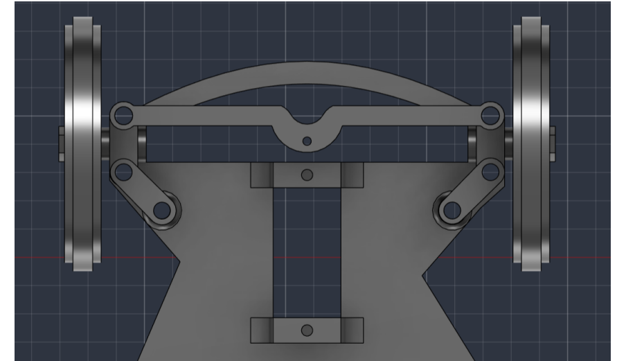
Front steering linkage, top view
