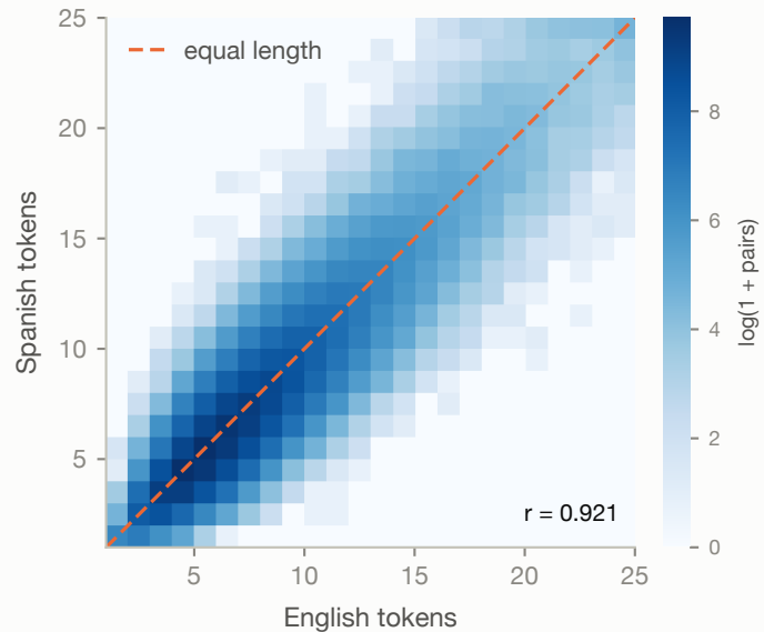
Source vs target length
