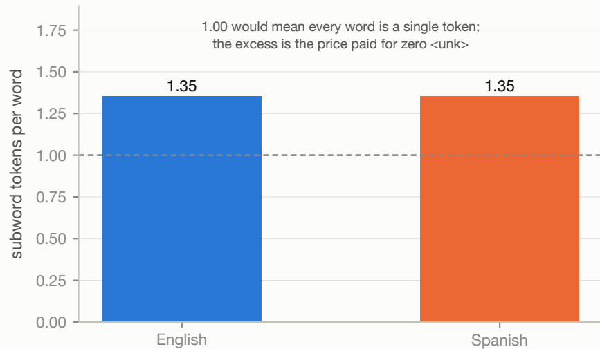
Fertility of the 16k joint BPE model
