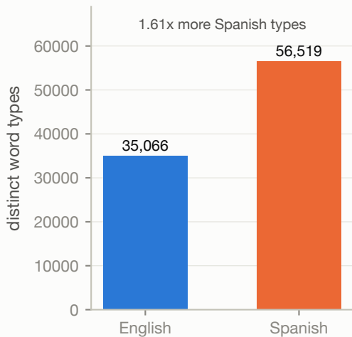
Vocabulary size
