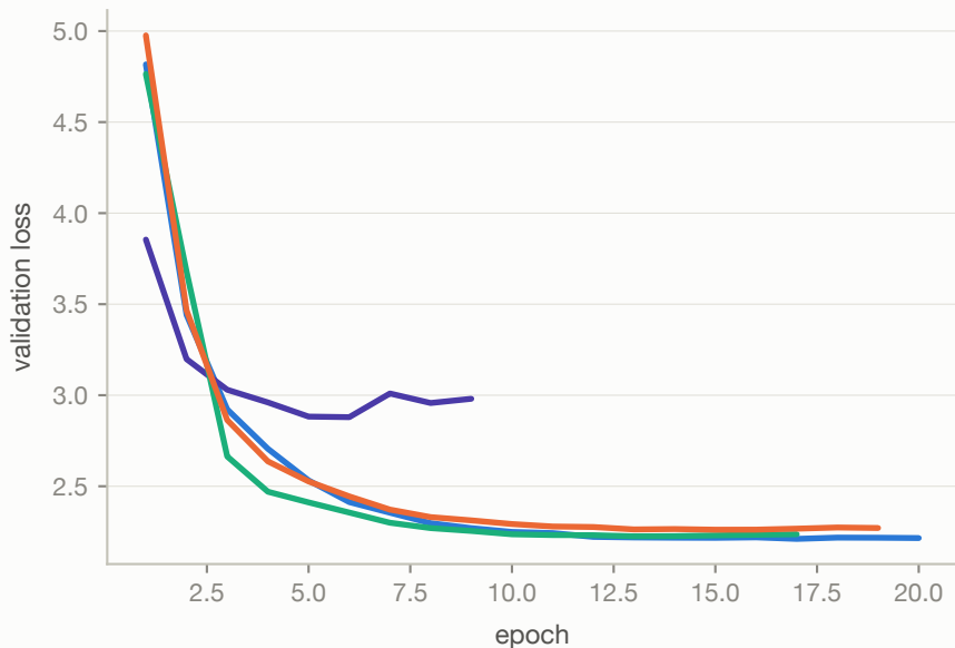
Validation loss
