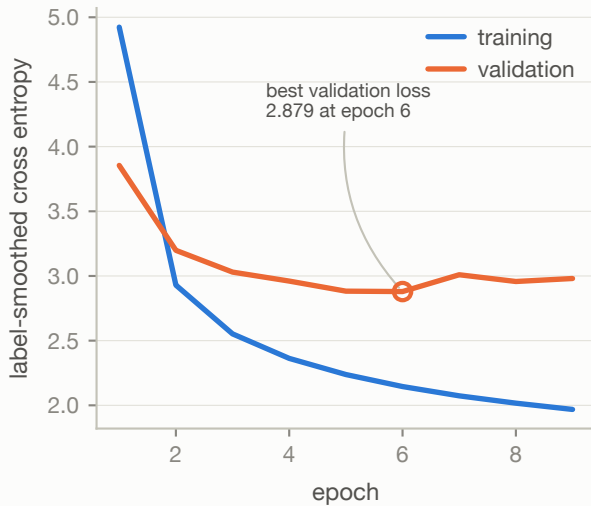
Loss
