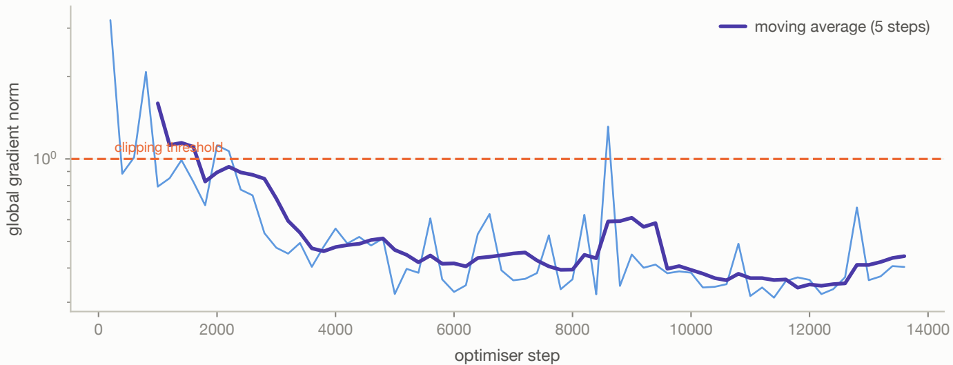
Gradient norms and the clipping threshold
