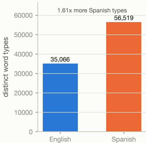
Vocabulary size
