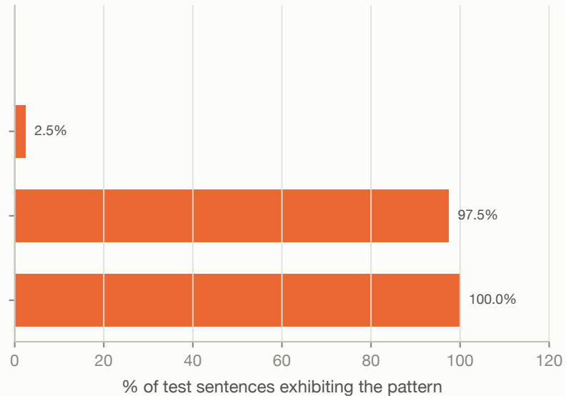
Spanish -> English
