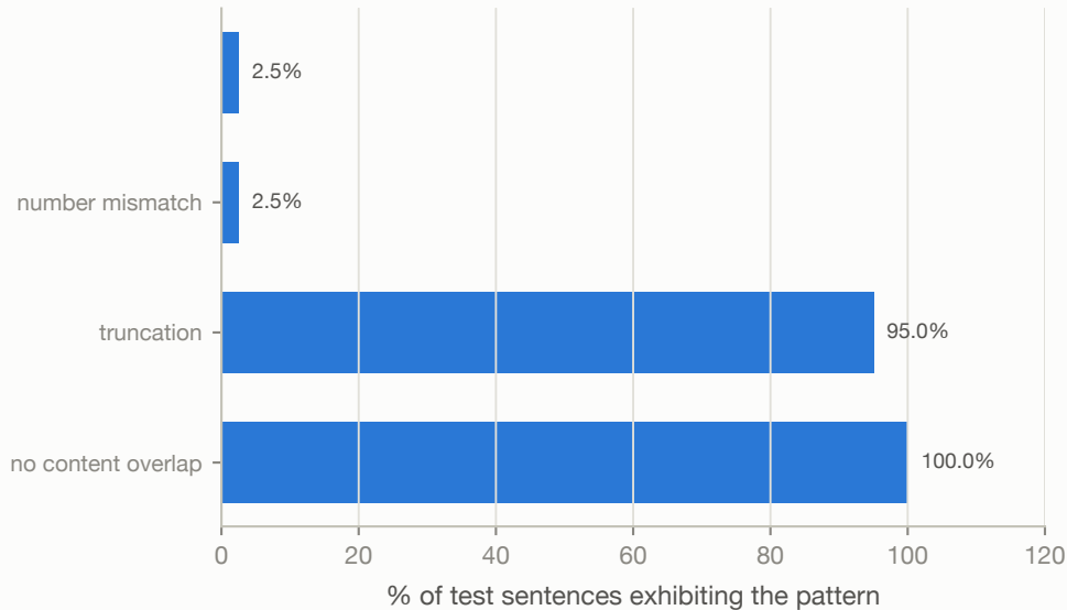
English -> Spanish
