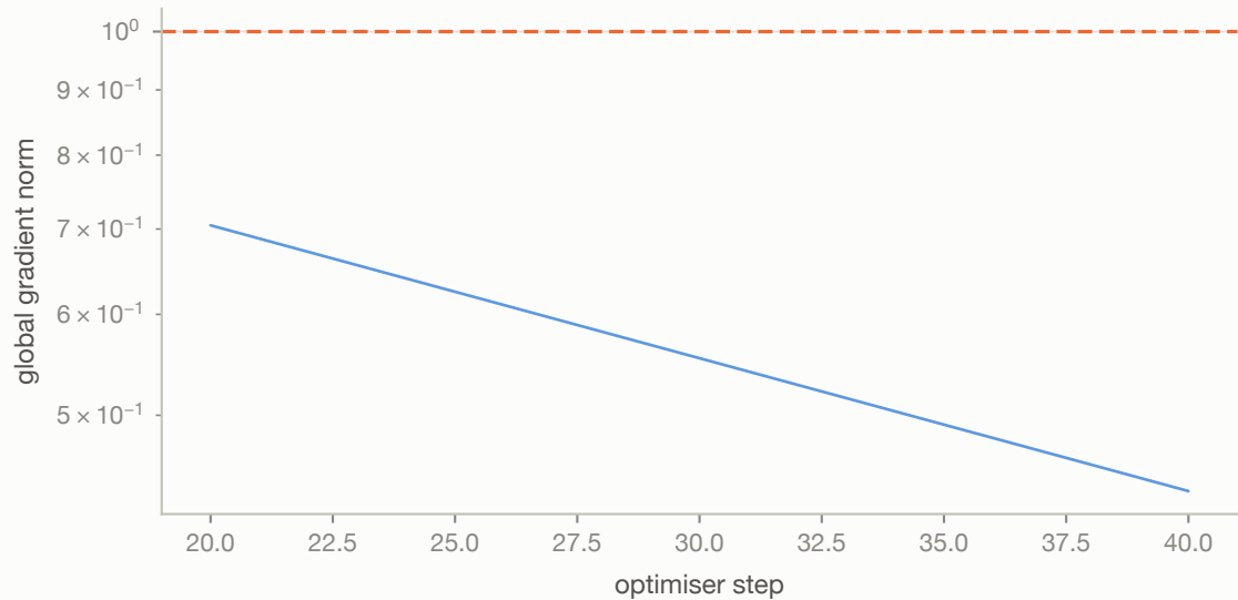
Gradient norms and the clipping threshold
