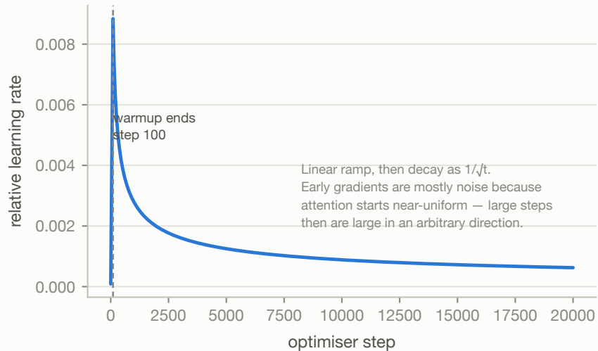
Inverse-square-root schedule
