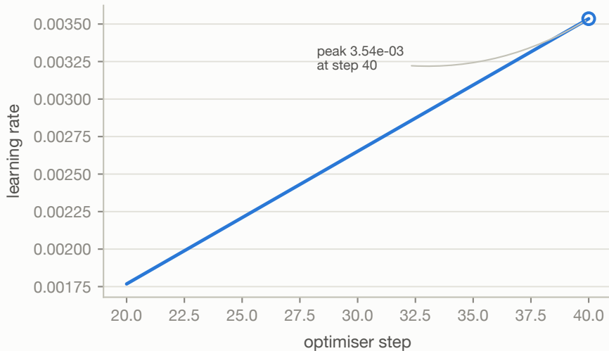
Realised schedule
