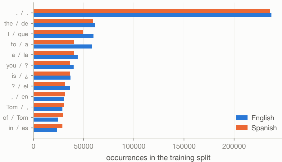
Most frequent tokens (English / Spanish)
