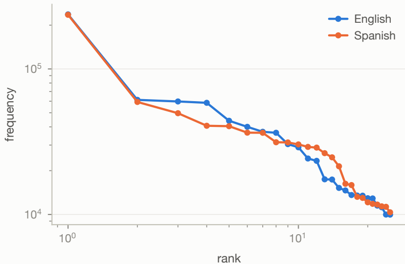
Top-25 tokens follow Zipf's law
