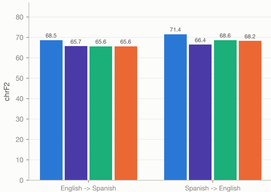
chrF2 on the held-out test set
