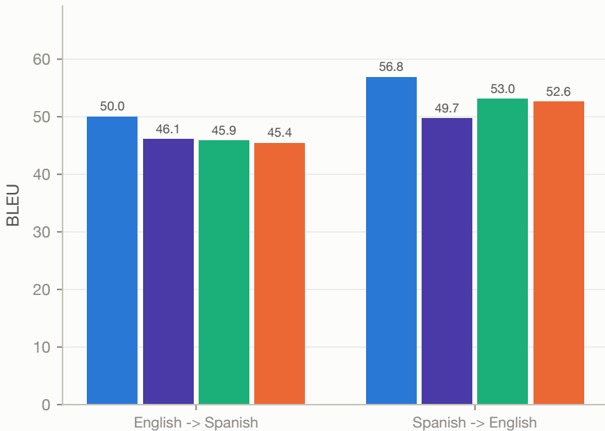
BLEU on the held-out test set
