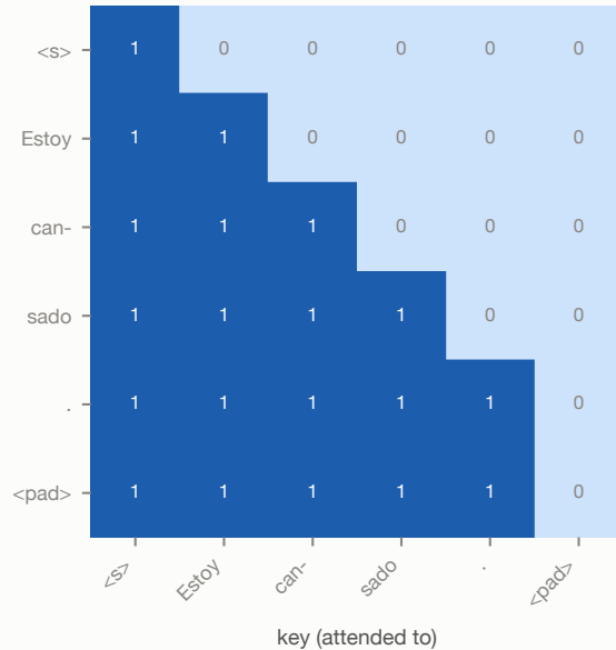
Combined (decoder self-attention)
