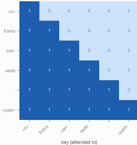
Causal mask
